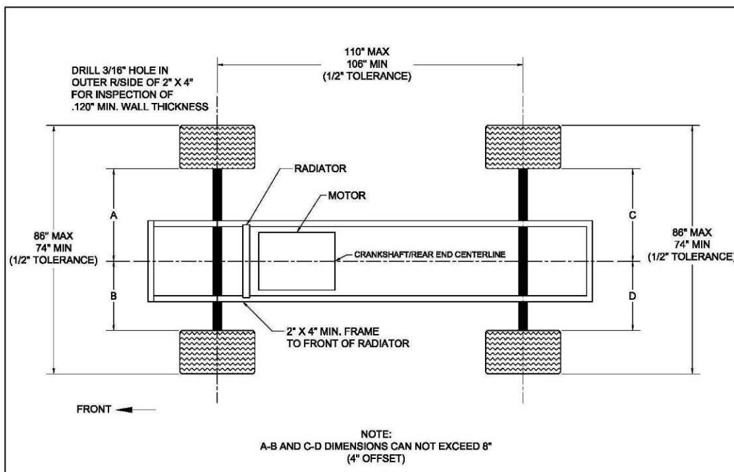
Transponder Location
