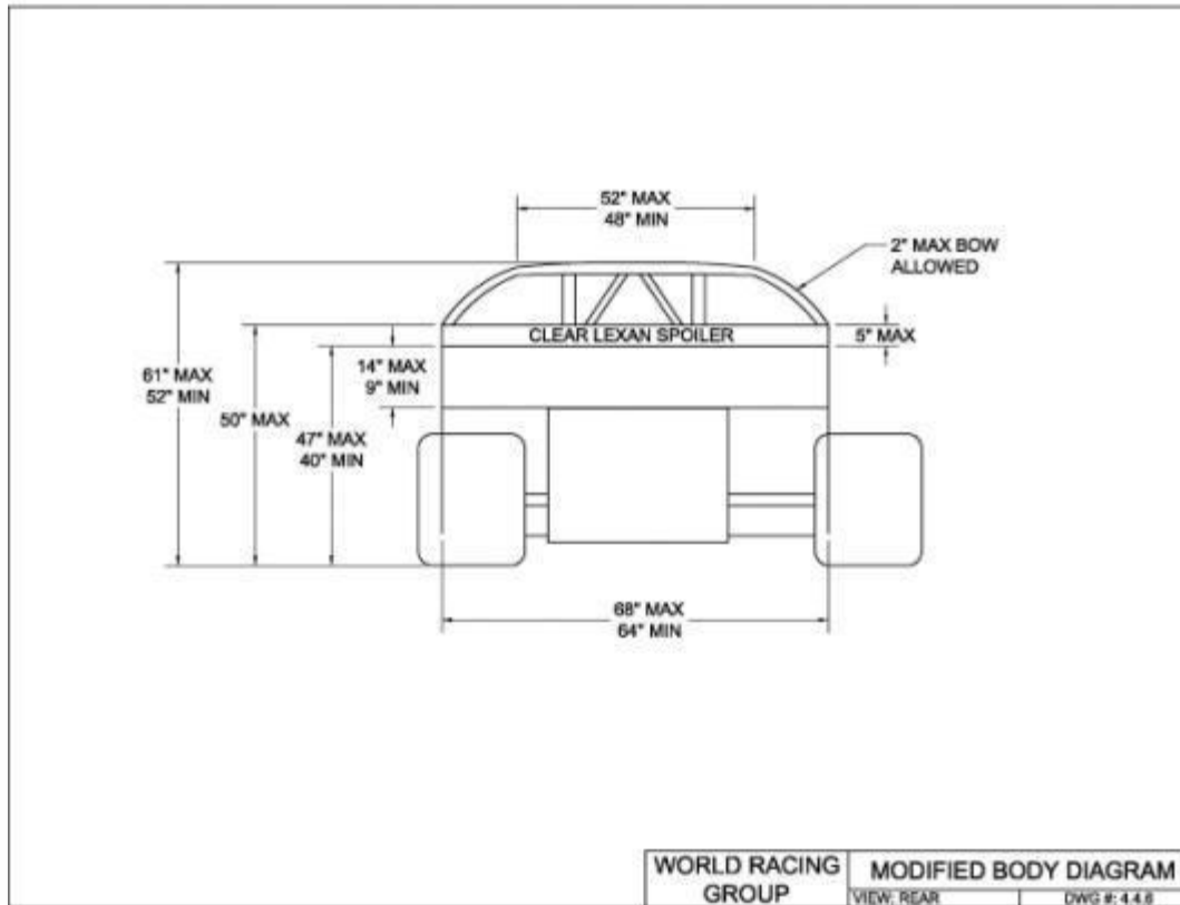
Chassis Diagram
